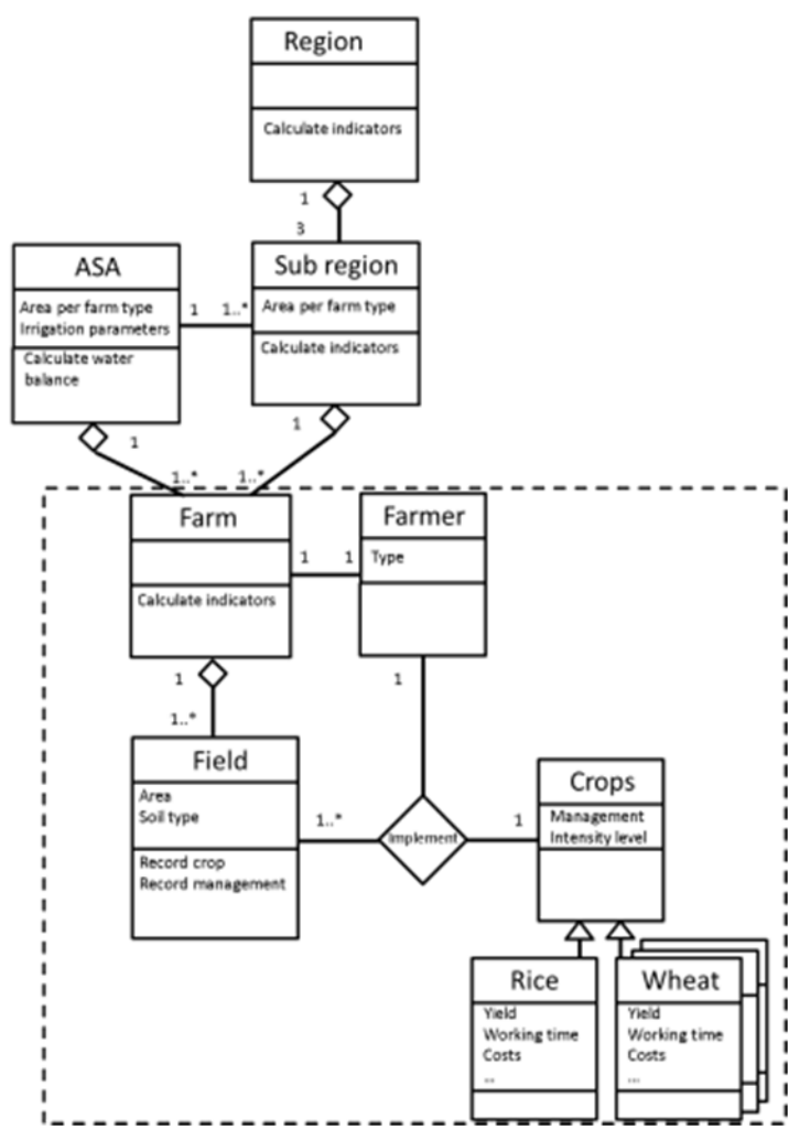
Figure 1: UML Class diagram of the IMPASIAS model.
